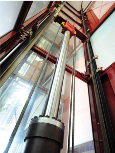
S-7 Hidrolik L Karkas L Frame For Hydraulic Lift
