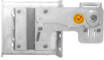
MK01 S STANDART KAYMA FREN STANDARD SLIP BRAKE
