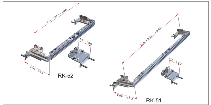
Ayarlanabilir Ahtapot Tipi Kuyu Arabölme Set-2 U Brackets Adjustable Shaft Divider Octopus Type Set-2
